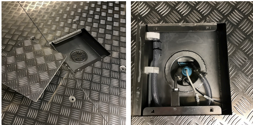
Figure 1 - Water drain
